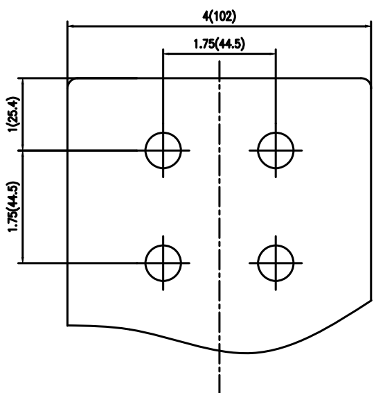
L.V. TERMINAL DETAIL
