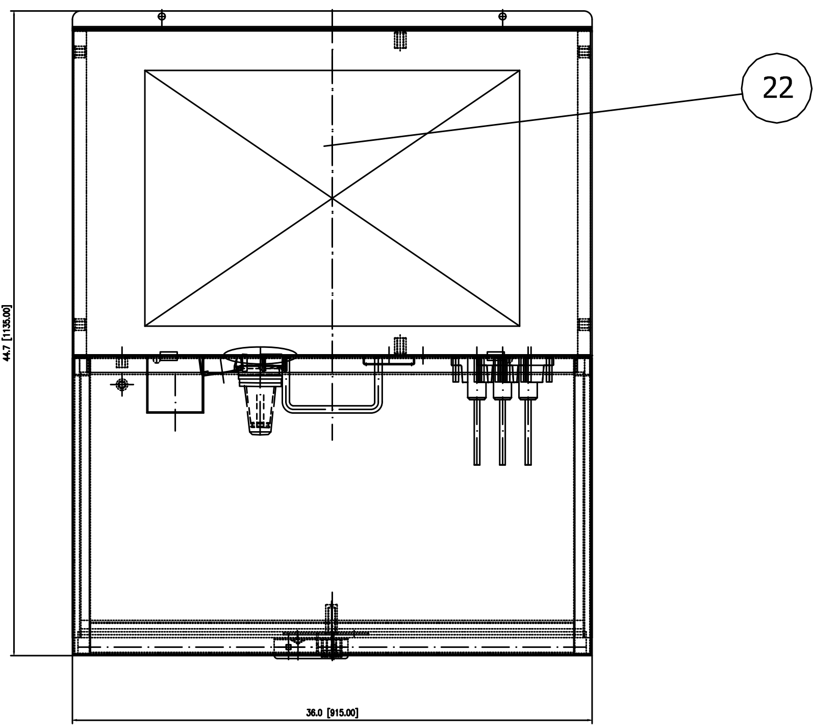
L.V. TERMINAL DETAIL
