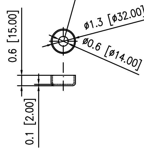
CUPPED WASHER DETAIL
