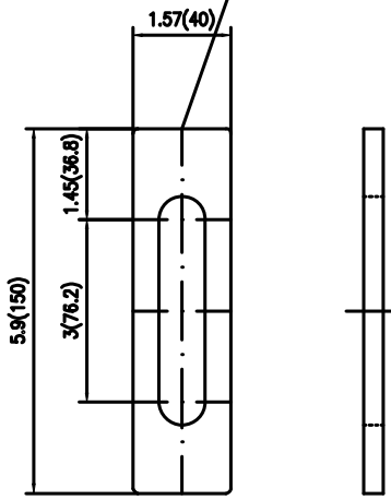
HOLD-DOWN PLATE DETAIL
